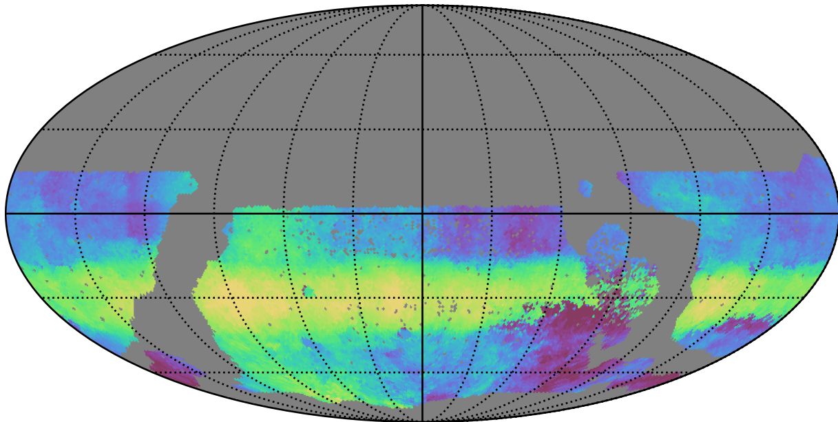
roman_v3.3_10yrs WFD r band: Median HA
