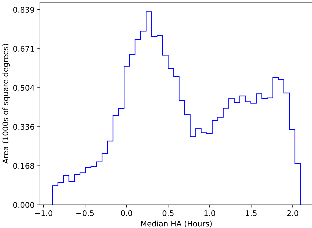
roman_v3.3_10yrs WFD r band: Median HA
