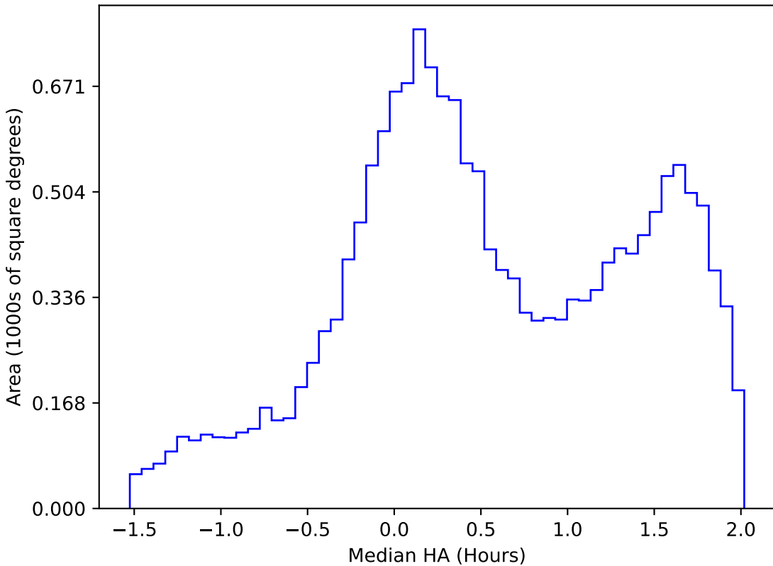
roman_v3.3_10yrs WFD g band: Median HA
