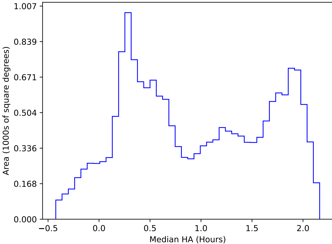
roman_v3.3_10yrs WFD all bands: Median HA
