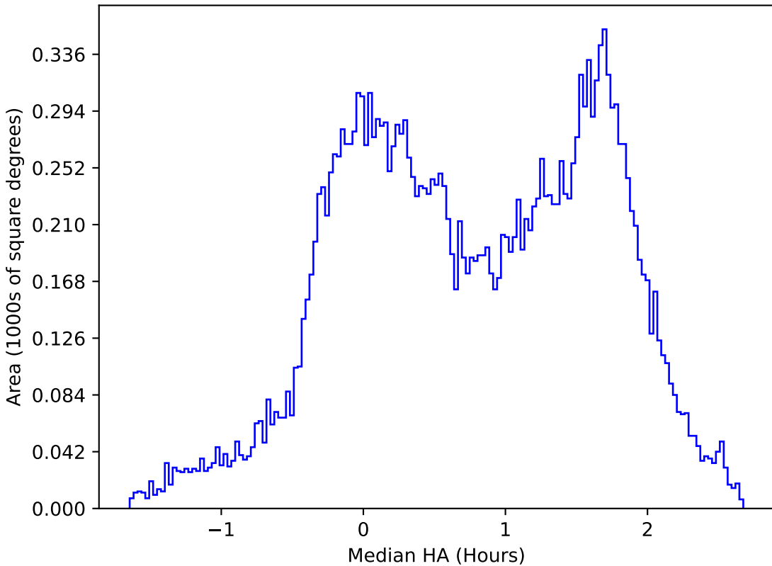
roman_v3.3_10yrs All sky u band: Median HA
