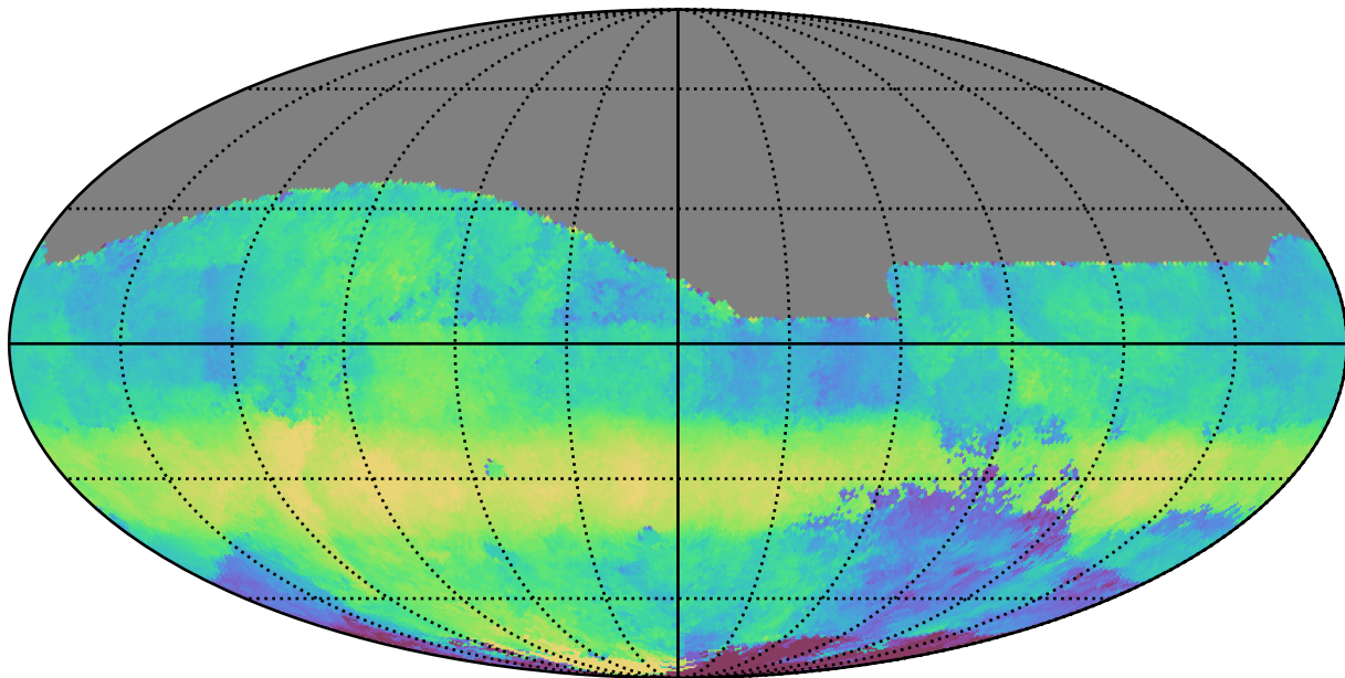
roman_v3.3_10yrs All sky r band: Median HA
