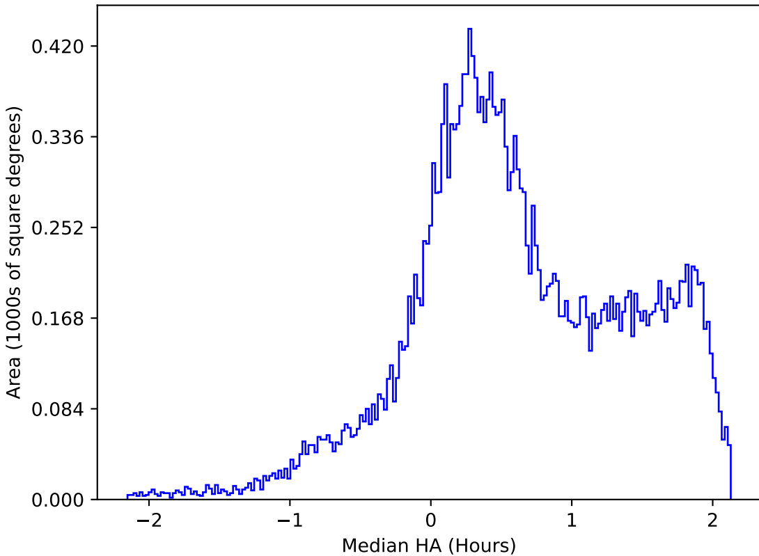
roman_v3.3_10yrs All sky r band: Median HA
