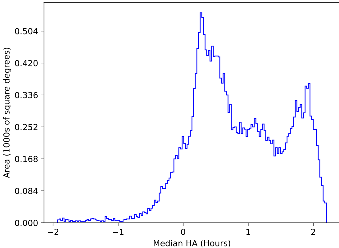
roman_v3.3_10yrs All sky all bands: Median HA
