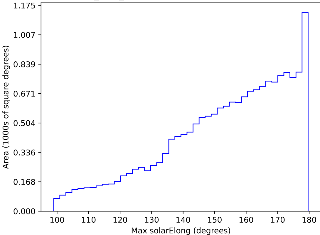
roman_v3.3_10yrs WFD all bands: Max solarElong
