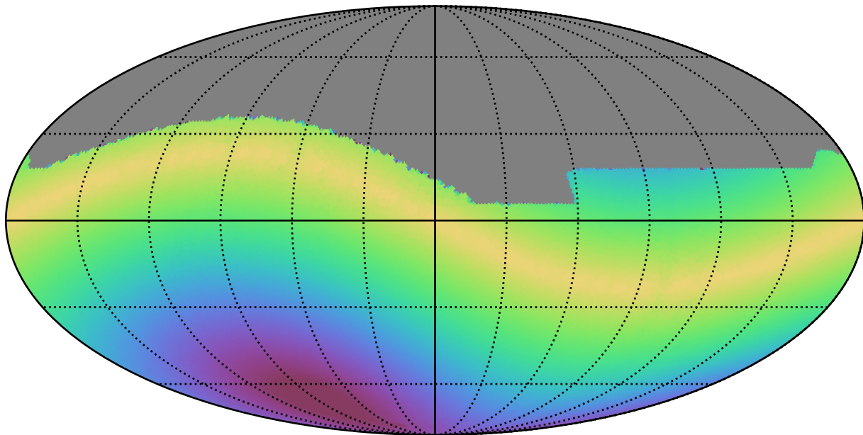
roman_v3.3_10yrs All sky all bands: Max solarElong
