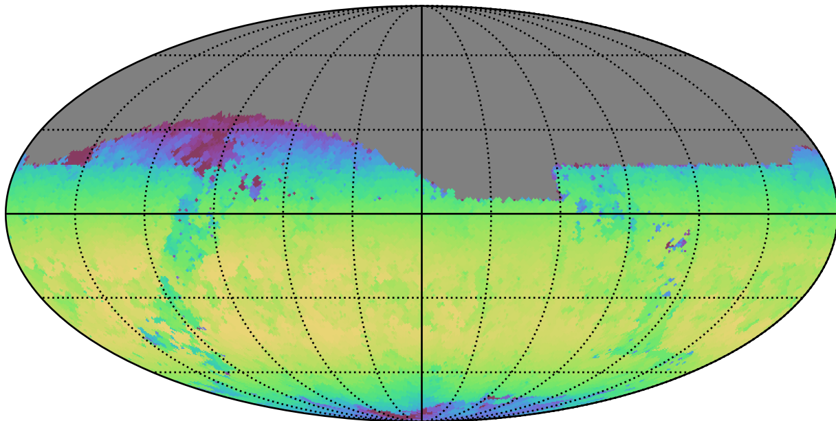
roman_v3.3_10yrs Yr 1 z band: Max skyBrightness
