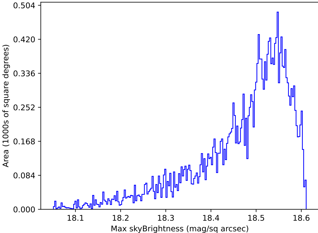
roman_v3.3_10yrs Yr 1 y band: Max skyBrightness
