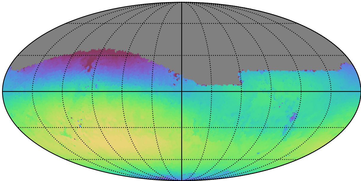
roman_v3.3_10yrs Yr 1 r band: Max skyBrightness
