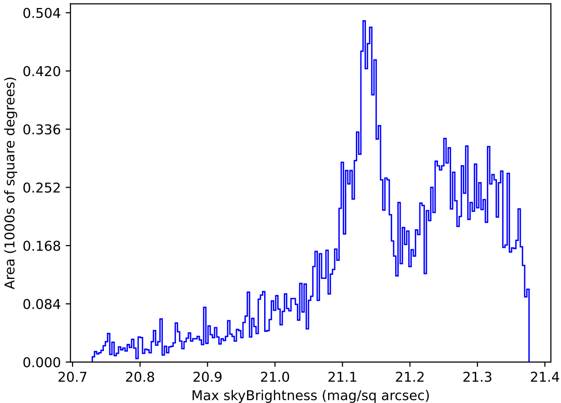
roman_v3.3_10yrs Yr 1 r band: Max skyBrightness
