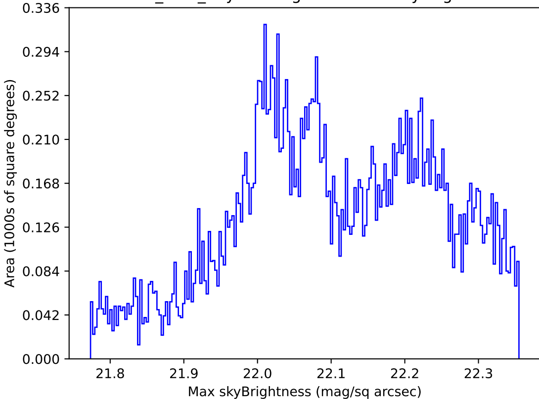
roman_v3.3_10yrs Yr 1 g band: Max skyBrightness
