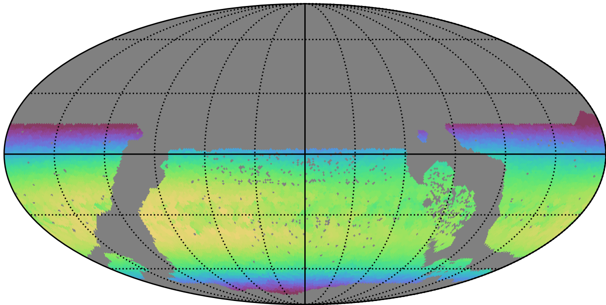
roman_v3.3_10yrs WFD z band: Max skyBrightness
