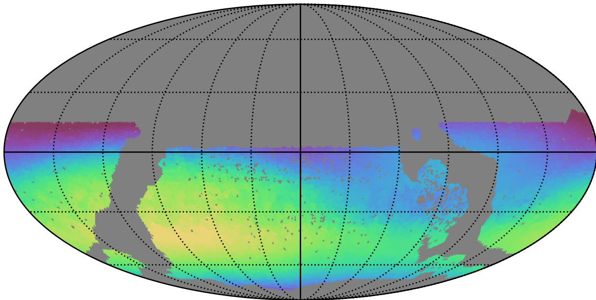
roman_v3.3_10yrs WFD u band: Max skyBrightness
