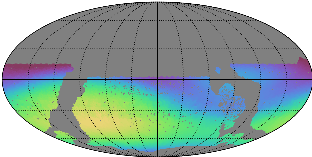
roman_v3.3_10yrs WFD r band: Max skyBrightness
