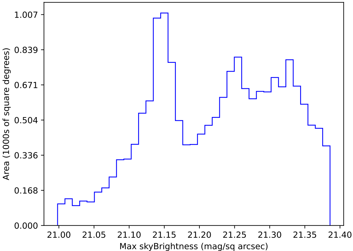
roman_v3.3_10yrs WFD r band: Max skyBrightness
