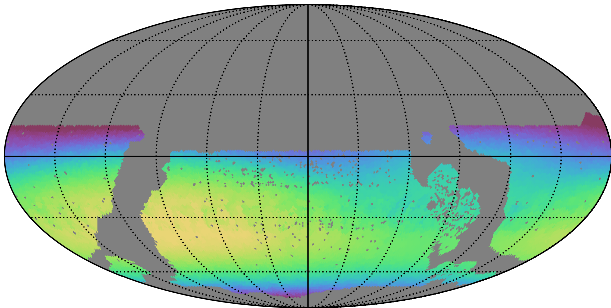
roman_v3.3_10yrs WFD i band: Max skyBrightness
