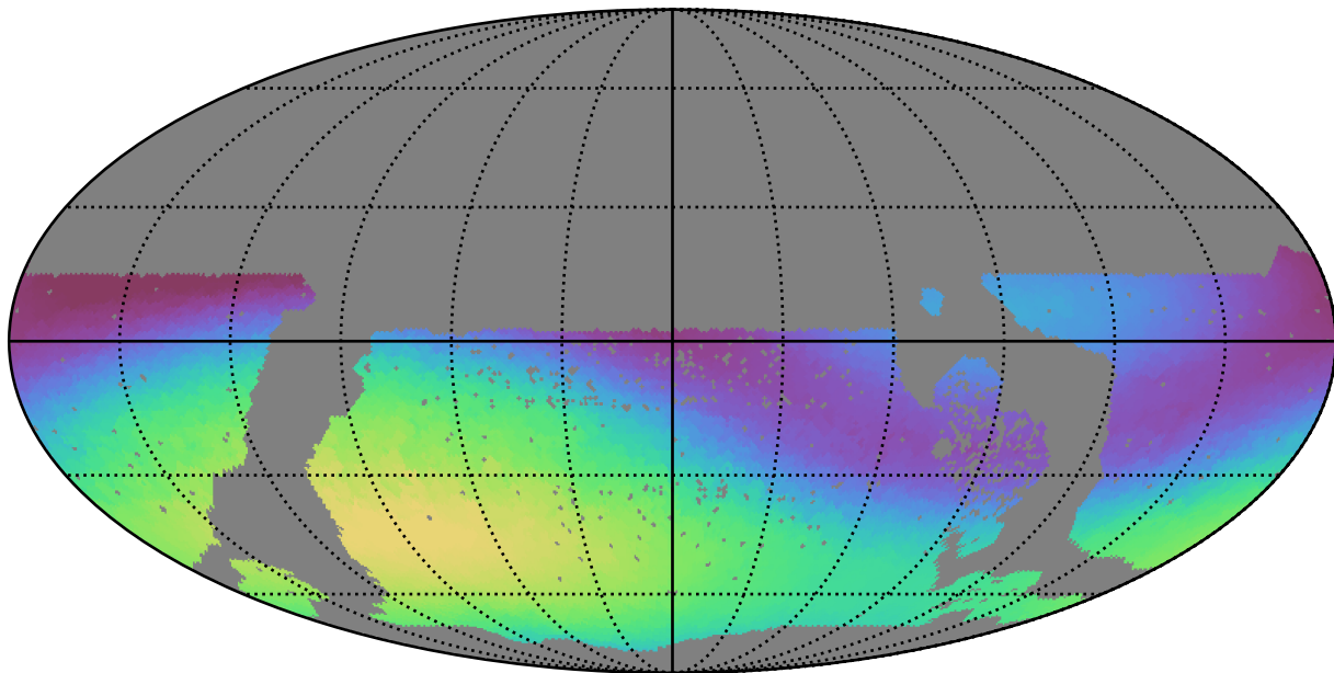
roman_v3.3_10yrs WFD g band: Max skyBrightness
