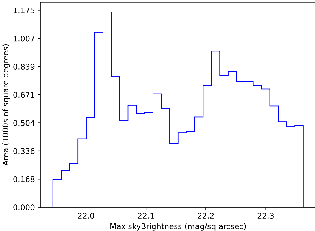
roman_v3.3_10yrs WFD g band: Max skyBrightness
