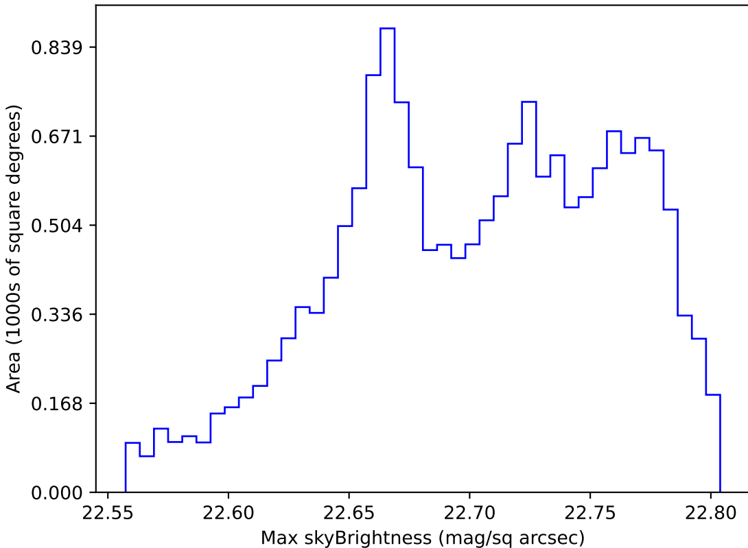
roman_v3.3_10yrs WFD all bands: Max skyBrightness
