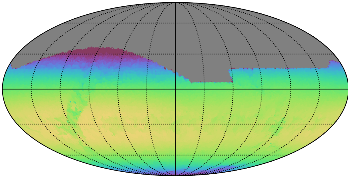
roman_v3.3_10yrs All sky z band: Max skyBrightness
