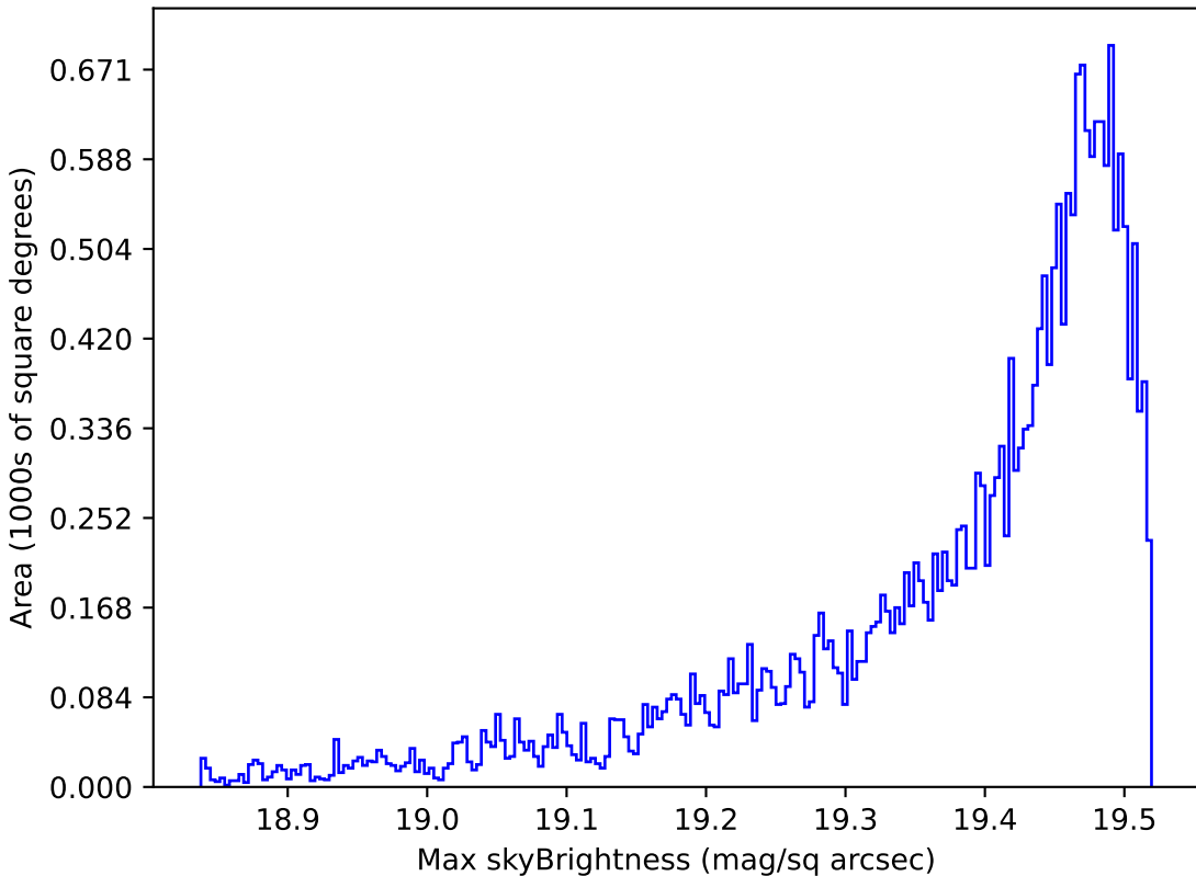
roman_v3.3_10yrs All sky z band: Max skyBrightness
