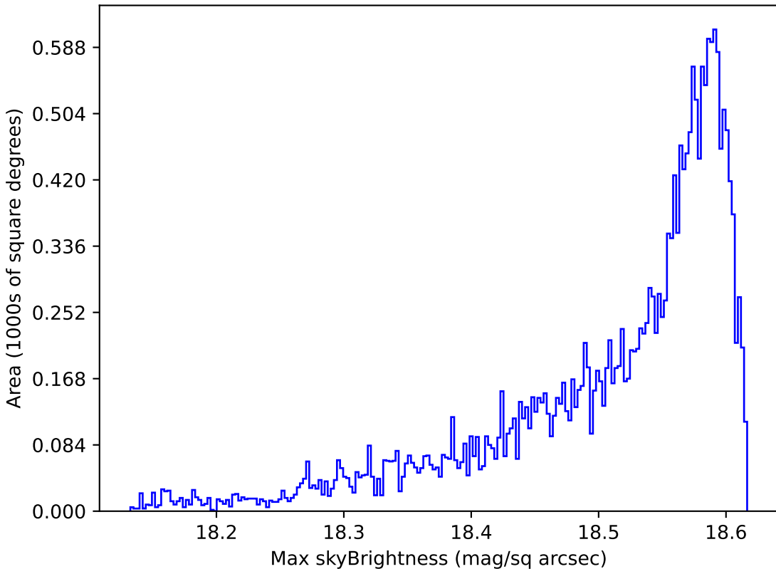
roman_v3.3_10yrs All sky y band: Max skyBrightness
