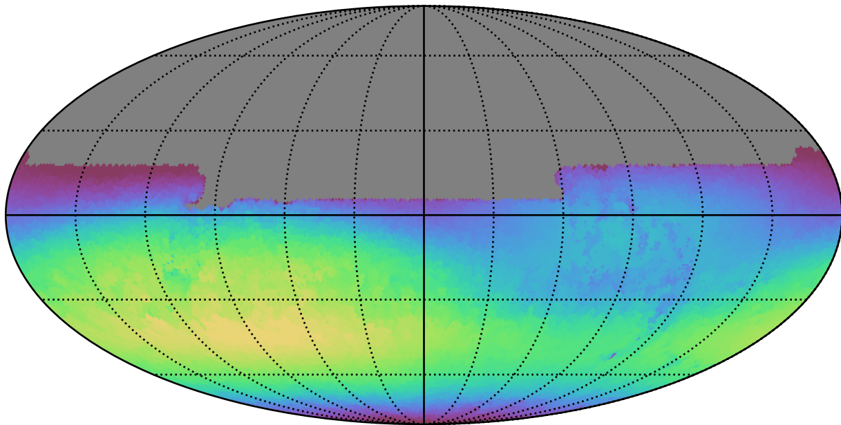
roman_v3.3_10yrs All sky u band: Max skyBrightness
