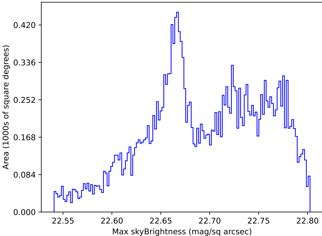
roman_v3.3_10yrs All sky u band: Max skyBrightness
