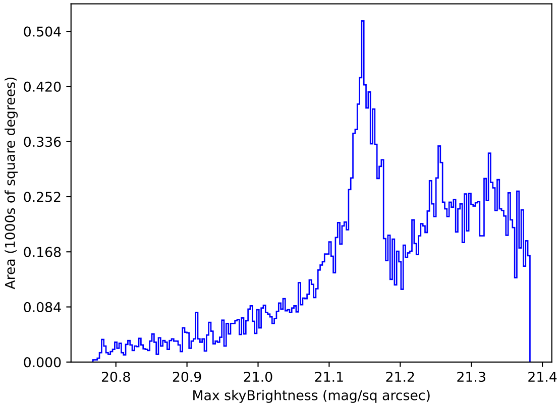
roman_v3.3_10yrs All sky r band: Max skyBrightness
