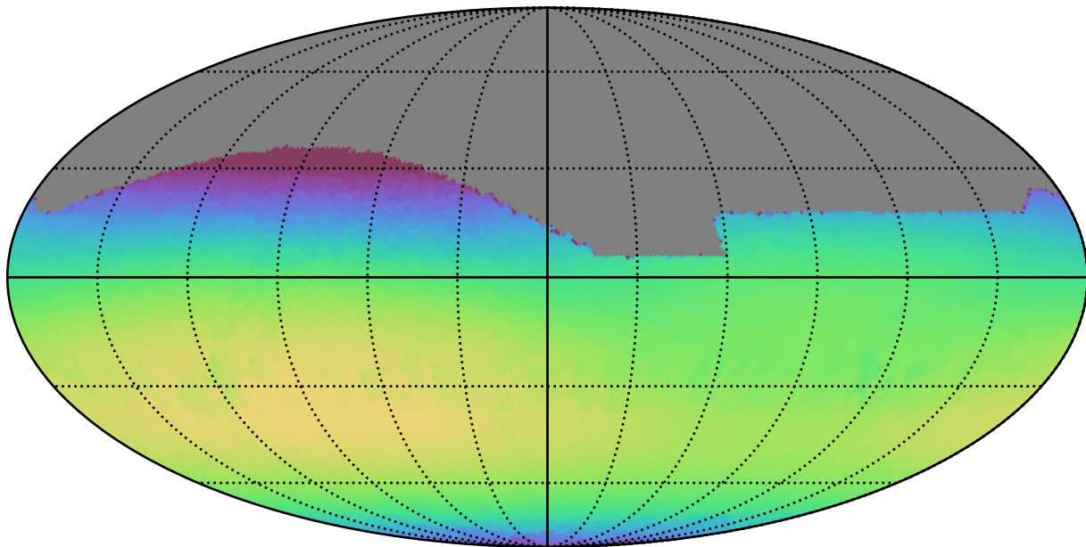
roman_v3.3_10yrs All sky i band: Max skyBrightness
