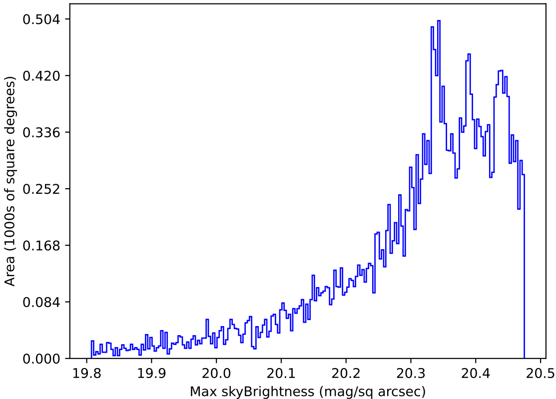
roman_v3.3_10yrs All sky i band: Max skyBrightness
