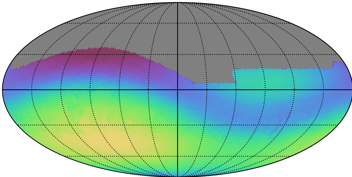
roman_v3.3_10yrs All sky g band: Max skyBrightness
