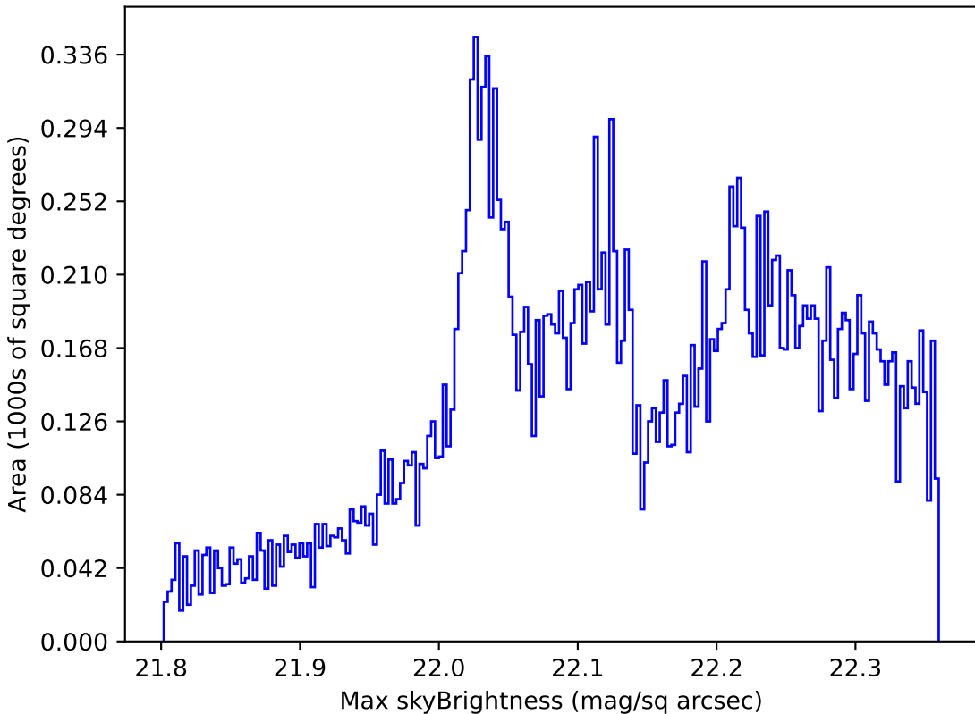
roman_v3.3_10yrs All sky g band: Max skyBrightness
