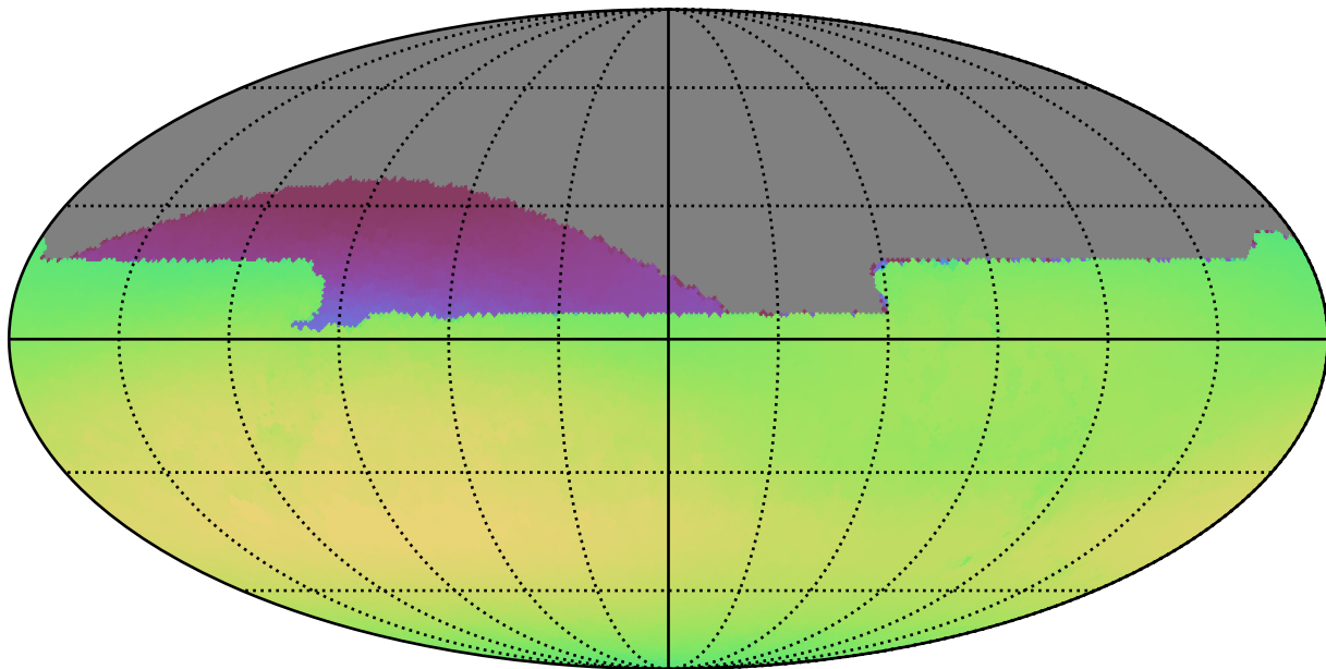
roman_v3.3_10yrs All sky all bands: Max skyBrightness
