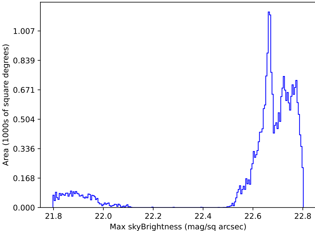
roman_v3.3_10yrs All sky all bands: Max skyBrightness
