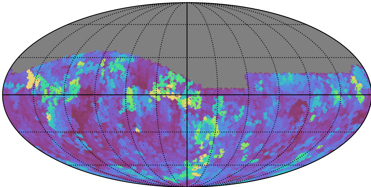
roman_v3.3_10yrs Yr 1 z band: Max seeingGeom
