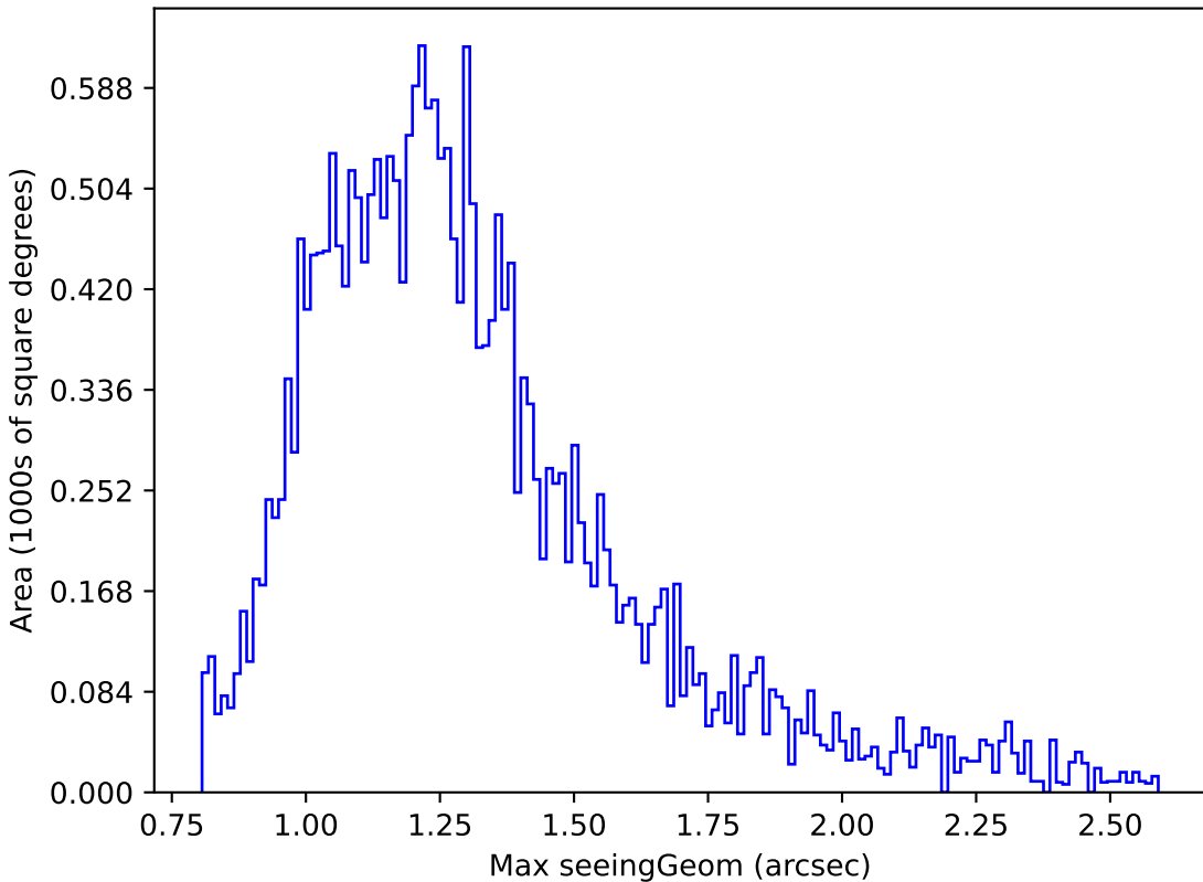
roman_v3.3_10yrs Yr 1 z band: Max seeingGeom
