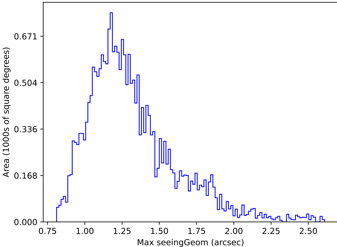
roman_v3.3_10yrs Yr 1 u band: Max seeingGeom
