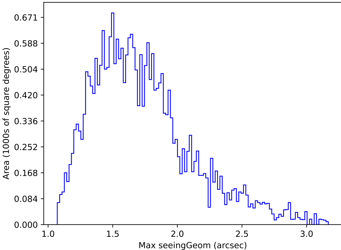
roman_v3.3_10yrs Yr 1 all bands: Max seeingGeom
