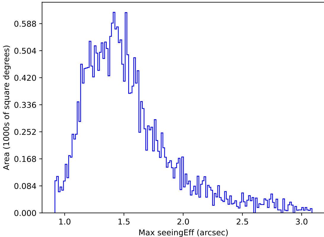
roman_v3.3_10yrs Yr 1 z band: Max seeingEff
