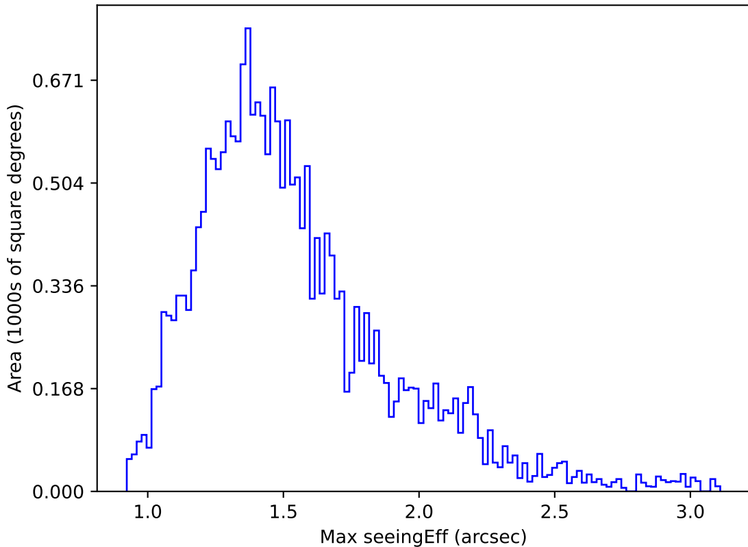
roman_v3.3_10yrs Yr 1 u band: Max seeingEff
