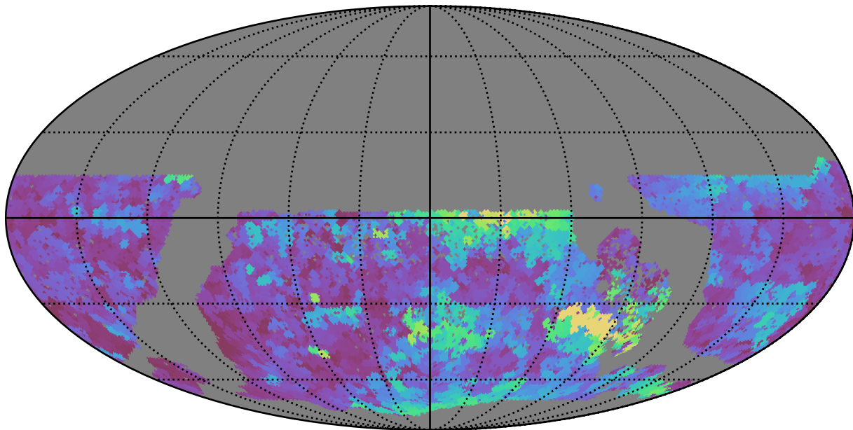
roman_v3.3_10yrs WFD u band: Max seeingEff
