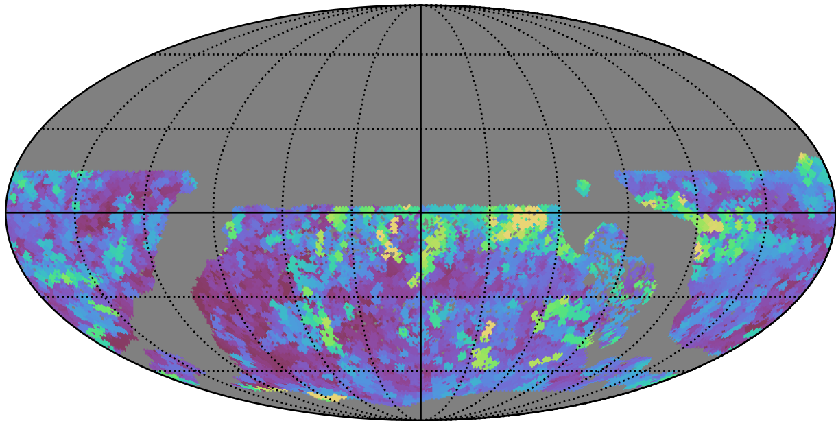
roman_v3.3_10yrs WFD r band: Max seeingEff
