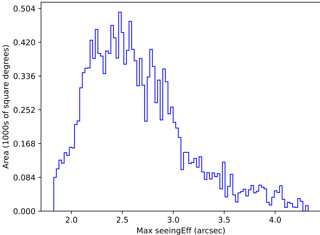
roman_v3.3_10yrs WFD r band: Max seeingEff
