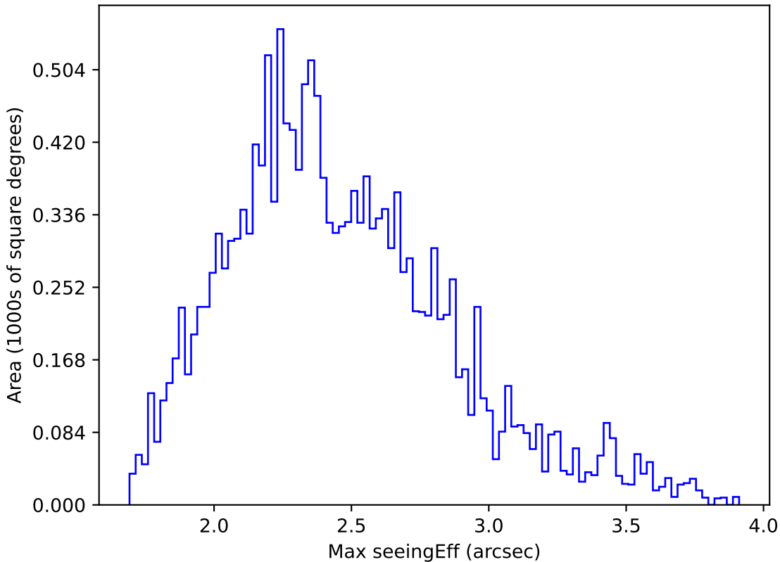
roman_v3.3_10yrs WFD g band: Max seeingEff
