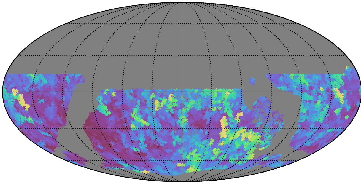
roman_v3.3_10yrs WFD all bands: Max seeingEff
