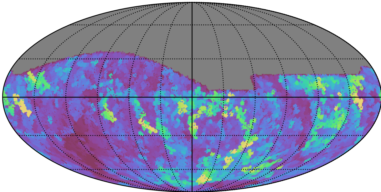
roman_v3.3_10yrs All sky z band: Max seeingEff
