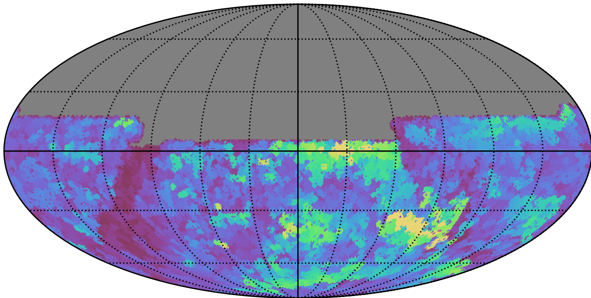
roman_v3.3_10yrs All sky u band: Max seeingEff
