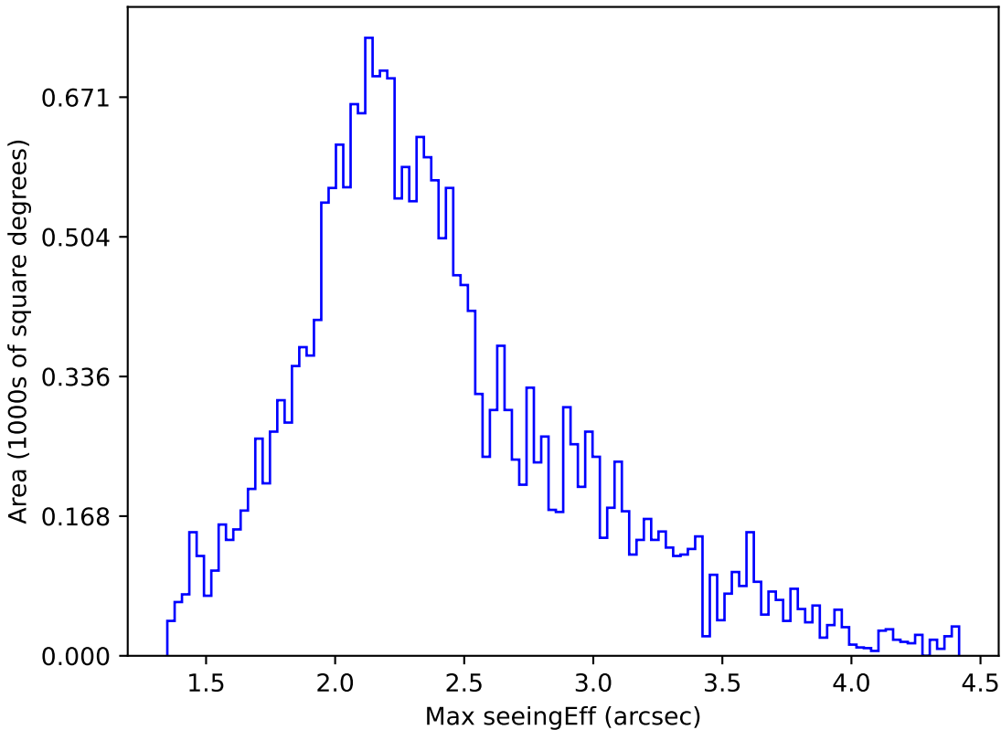
roman_v3.3_10yrs All sky u band: Max seeingEff
