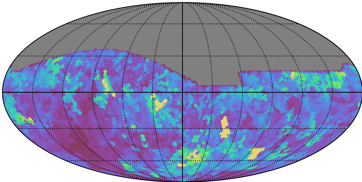
roman_v3.3_10yrs All sky i band: Max seeingEff
